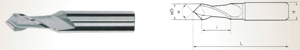
整體硬質合金倒角銑刀 Solid Carbide Chamfer mills
