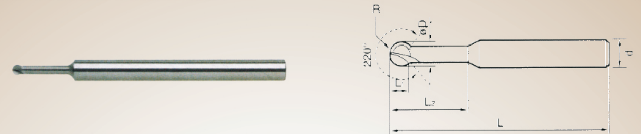
整體硬質合金220°球頭銑刀 Solid Carbide ball nose With 220°
