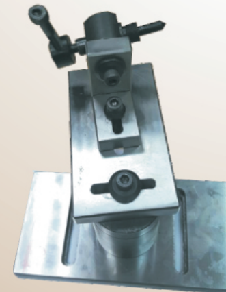
草轆機專用夾具 Grass reel machine fixture
