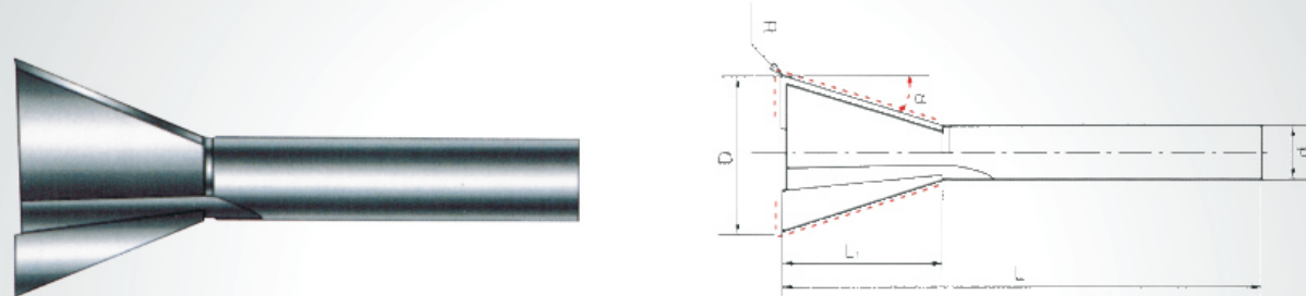
硬質合金燕尾槽銑刀 Solid Carbide Dov mills
